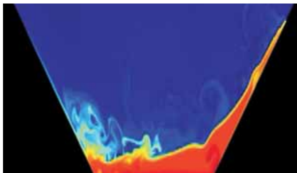
Complex numerical model calculated to match the 1958 Lituya Bay, Alaska landslide-generated local tsunami which caused the largest runup ever recorded (525 m). The complex model matches very closely the detail of the second order eddies and splash effects that laboratory experiments showed. Courtesy of Galen Gisler, Los Alamos National Laboratory.
