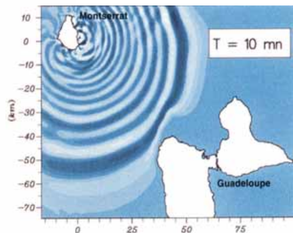
Numerical modelling snapshots of the water surface 10 minutes after a pyroclastic flow on the southeastern part of Montserrat Island led to a submarine landslide and the generation of a tsunami. Courtesy of LDG-France.
