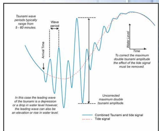
Mareogram (sea level) record of a tsunami.
