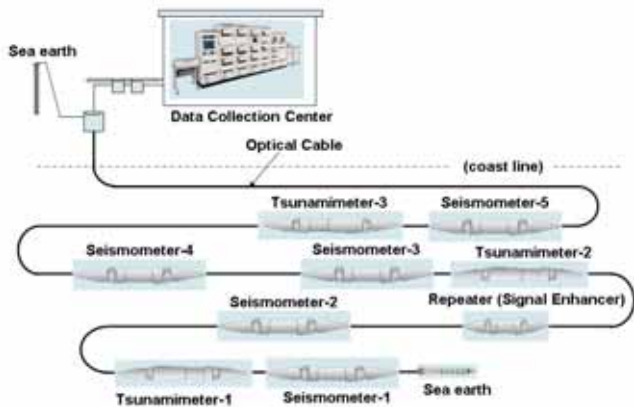
Schematic diagram of cabled ocean system for monitoring earthquakes and tsunamis. Courtesy of JMA.
